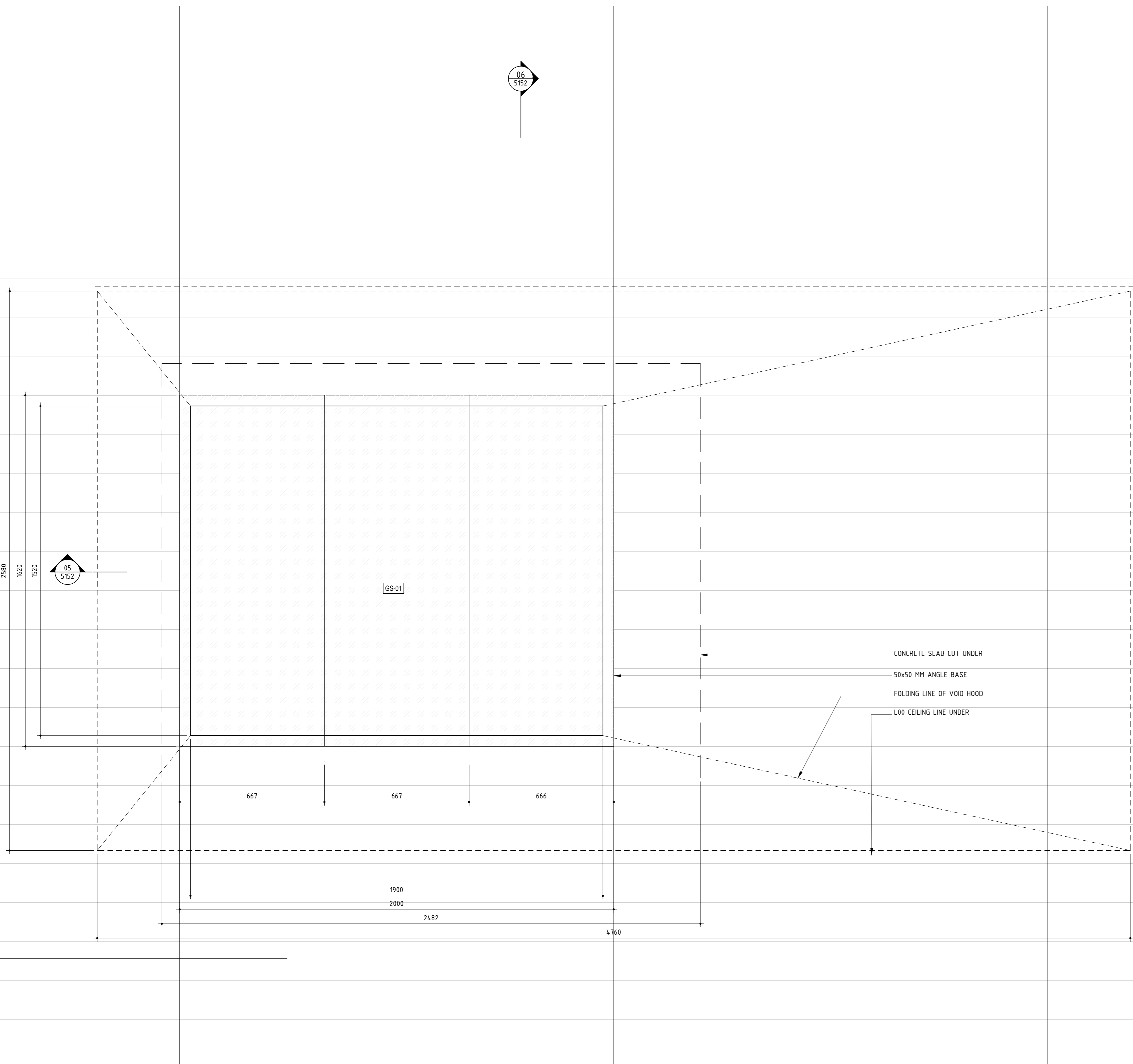
05 GLASS FLOOR AND VOID - PLAN SCALE 1:10
