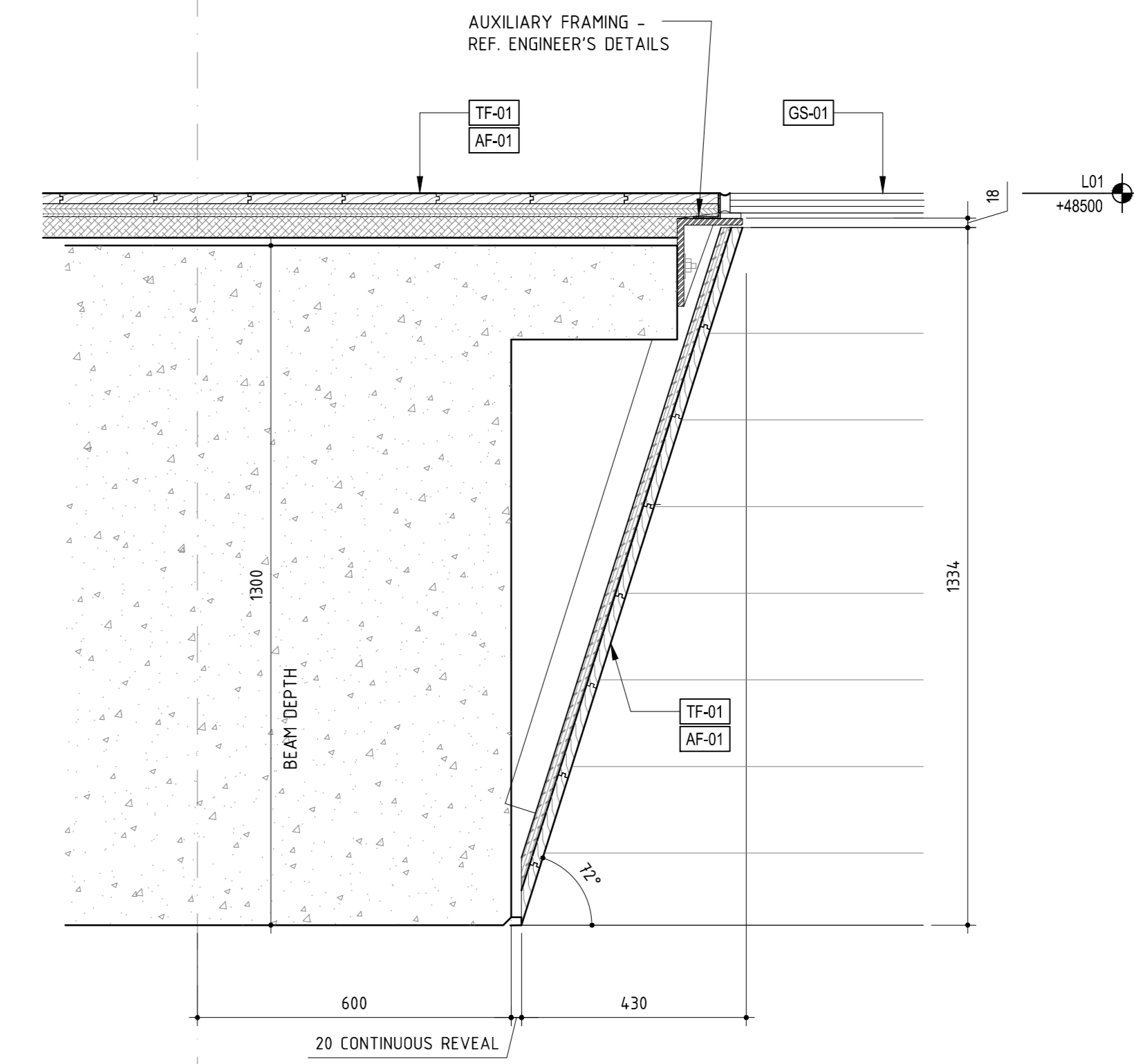
01 GLASS FLOOR AND VOID - SECTION SCALE 1:10
