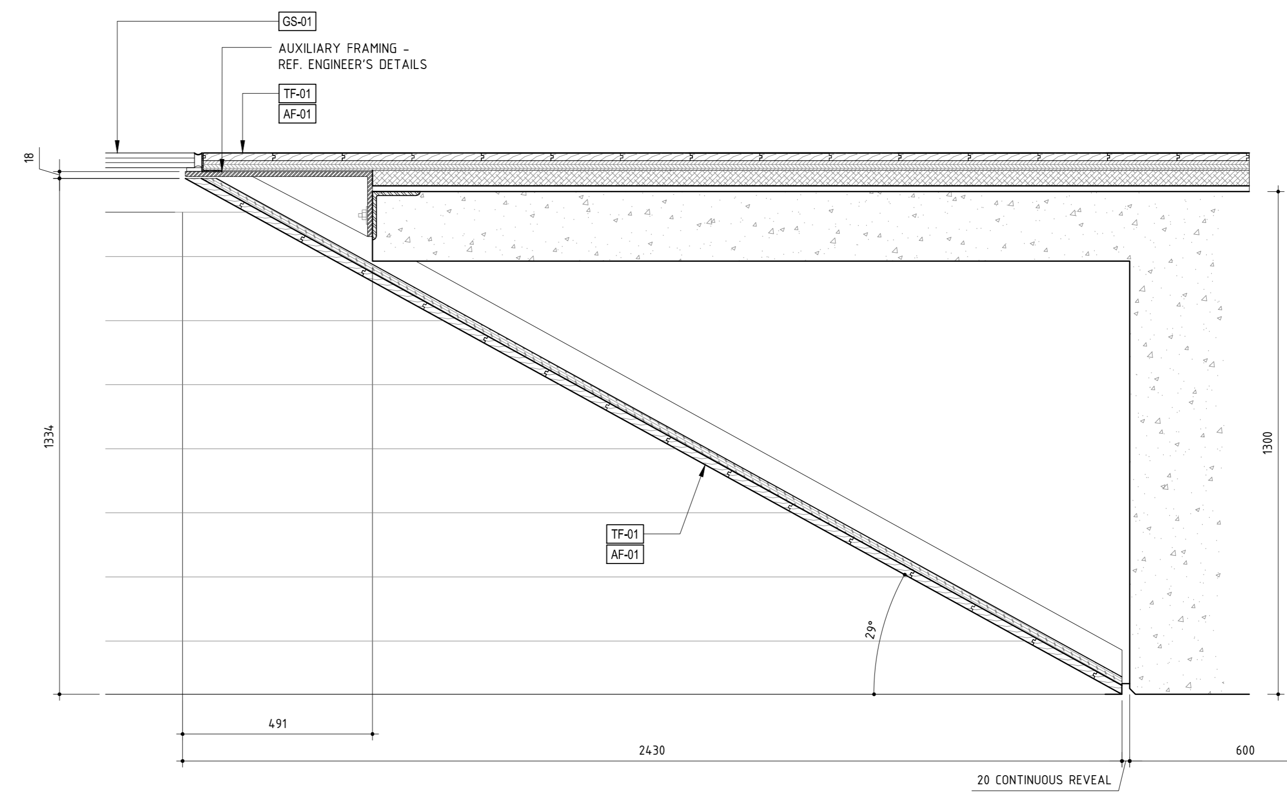
02 GLASS FLOOR AND VOID - SECTION SCALE 1:10
